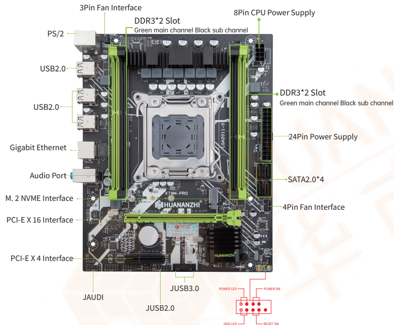
1-1 X79M PRO Motherboard illustration
